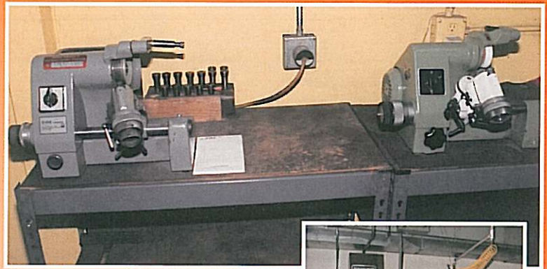
D-M-E CG-580 Cutter Grinder; GREPRUFTE SICHERHEIT/SIEMENS ILF5063-2AB93-Z Cutter Grinder
