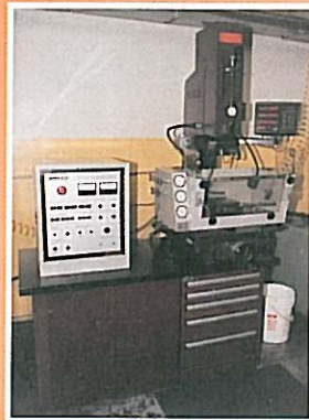
HANSVEDT Benchman EDM with H-Pulse 201 E Power Supply
